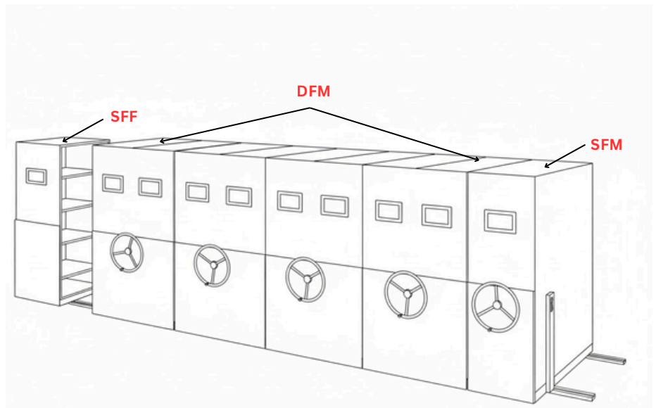
Isometric View
